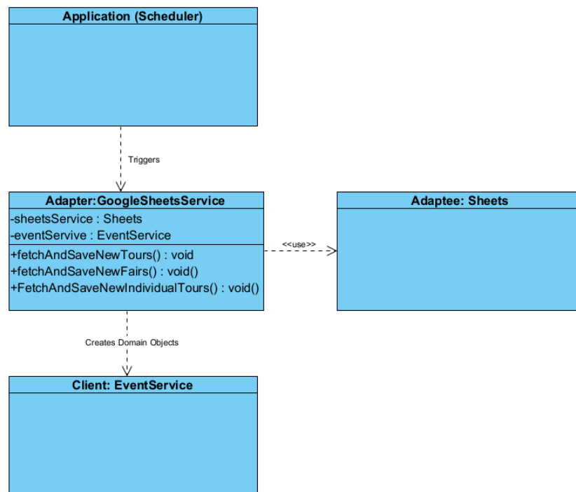
Figure 1: Isolated Illustration of Adapter Design Pattern for Better Visualization
